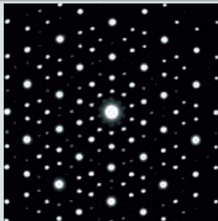
Dan Shechtman's diffraction pattern, figure: www.nobelprize.org
